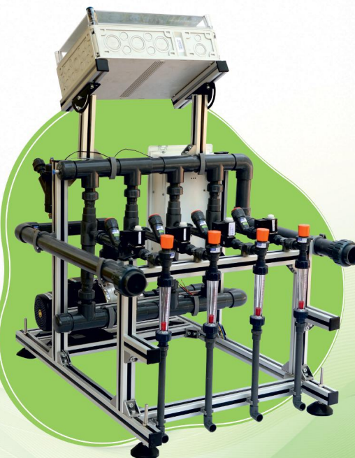
Fertigation Controller with Injector Unit
