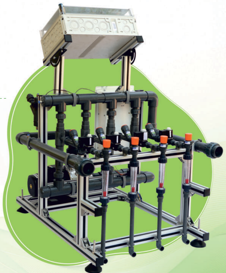
Fertigation Controller with Injector Unit
